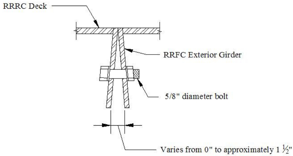
Figure B.3. Type 3 longitudinal flatcar connection (BCB3 & BCB5).
