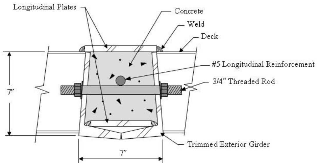
Figure B.2. Type 2 longitudinal flatcar connection (timber planking not shown) (WCB1, WCB2, & WCB3).
