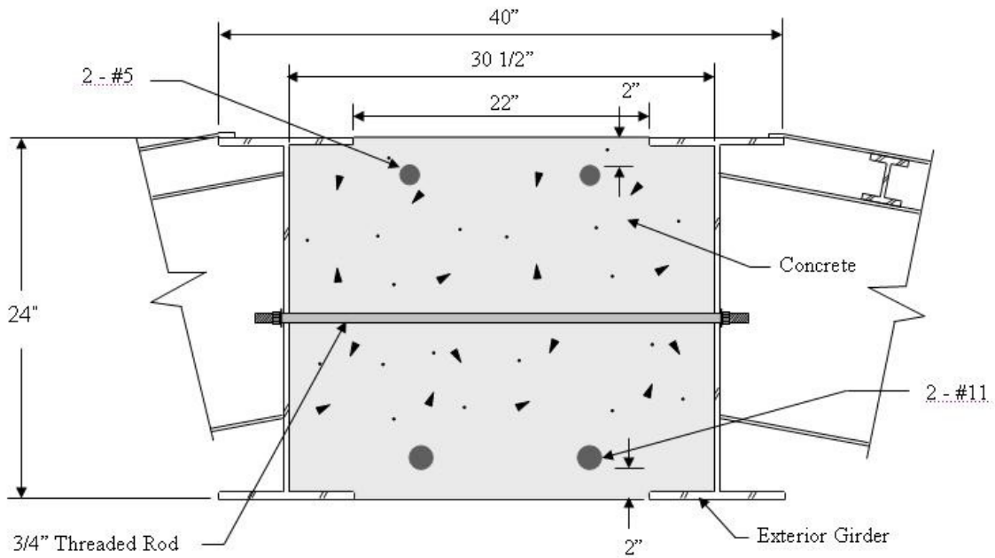
b. Wider Type 1 Connection used with 56-ft V deck RRFC (BCB2)
