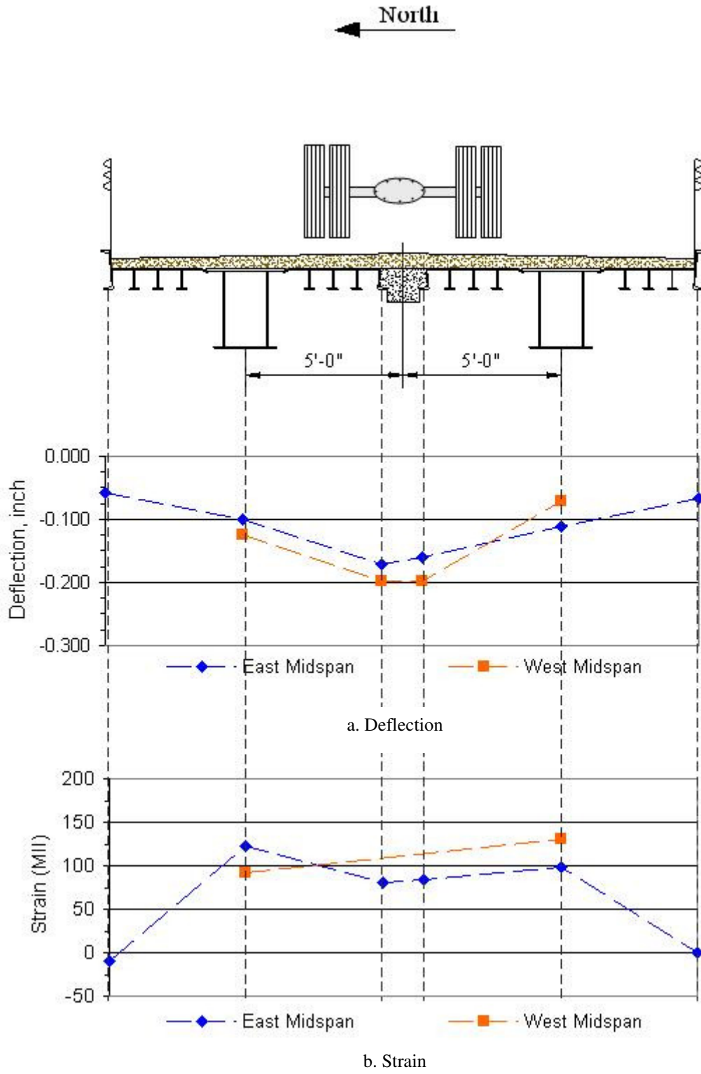
Figure 2.12. BCB4 Lane 2 midspan live load deflections and strains.
