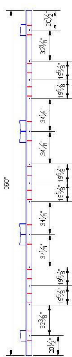
b. Approximate spacing of 3/4" bolts
