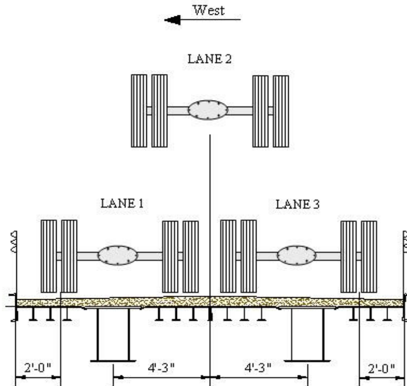
Figure 3.11. BCB5 lane configuration for load tests.
