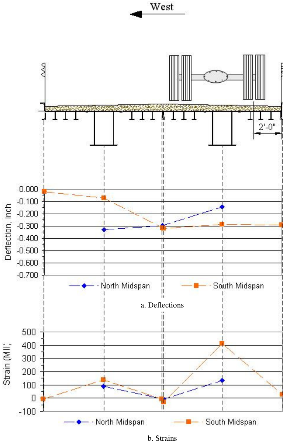
Figure 3.14. BCB5 Lane 3 midspan live load deflections and strains.
