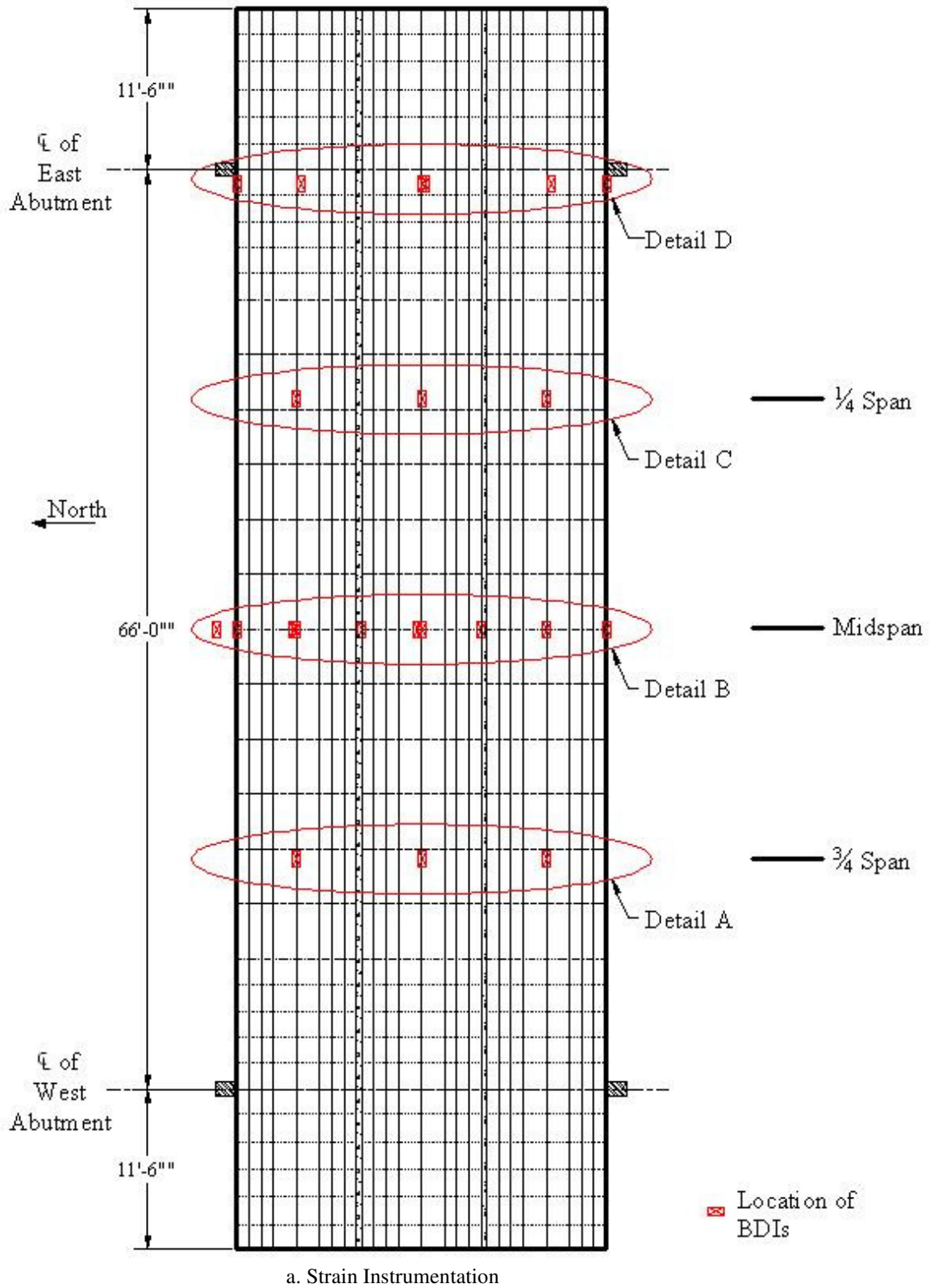
Figure 4.7. WCB3 instrumentation plan.
