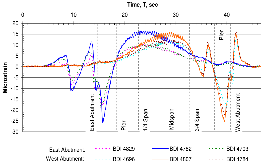
Figure A.18. Strain comparison for east and west abutments.
