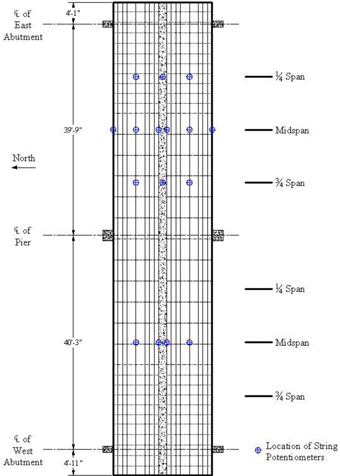
1. Deflection Instrumentation
