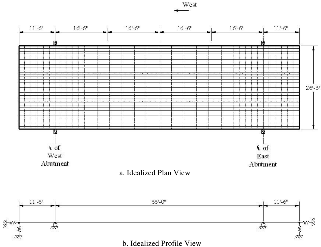
Figure 4.3. Idealized layout of WCB3.
